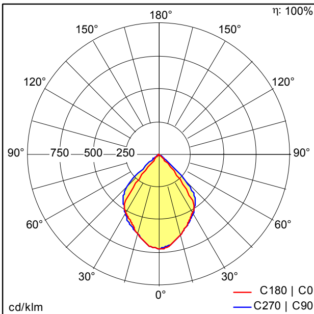
TE_HOLLY_CONE_DOWN_IP65_300_830.ltd
